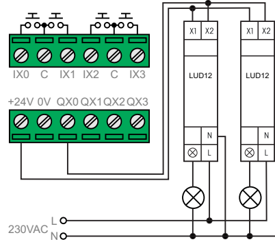
Power increased with a parallel connection of drivers
