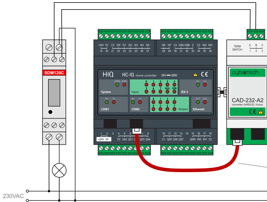
SDM-120C power meter
