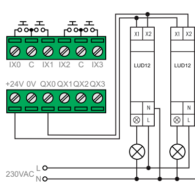
Power increased with a parallel connection of drivers
